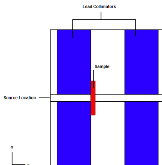
Figure 2.2 Simulation setup for MCNP calculations
