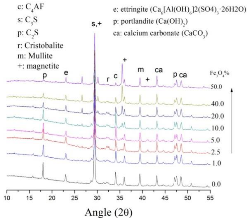
Figure 3.5 XRD patterns for white ordinary Portland cement paste with magnetite
