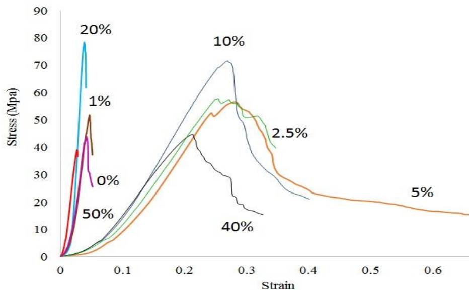
Figure 3.2 Typical stress-strain curves for the cement-magnetite composites
